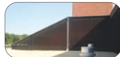
Above, Sentex SL580 operators power the four slide gates on the project. Shown below is a portion of the 579 linear feet of 16-foot-high mini-mesh chain link which was installed on the roofs of three of the buildings to keep birds out.
