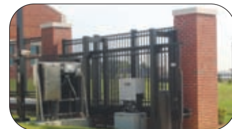
Above, Sentex SL580 operators power the four slide gates on the project. Shown below is a portion of the 579 linear feet of 16-foot-high mini-mesh chain link which was installed on the roofs of three of the buildings to keep birds out.
